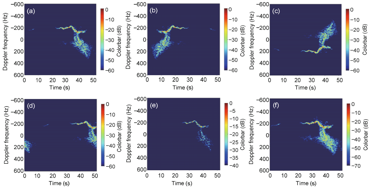
Fig. 7 Time-frequency images via data augmentation: (a) original image; (b) image via left-right flipping; (c) image via up-down flipping; (d) result of the sampling-based data augmentation method; (e) result of setting the SNR within [-40, 0] dB; (f) result of setting the SNR within [-70, 0] dB
